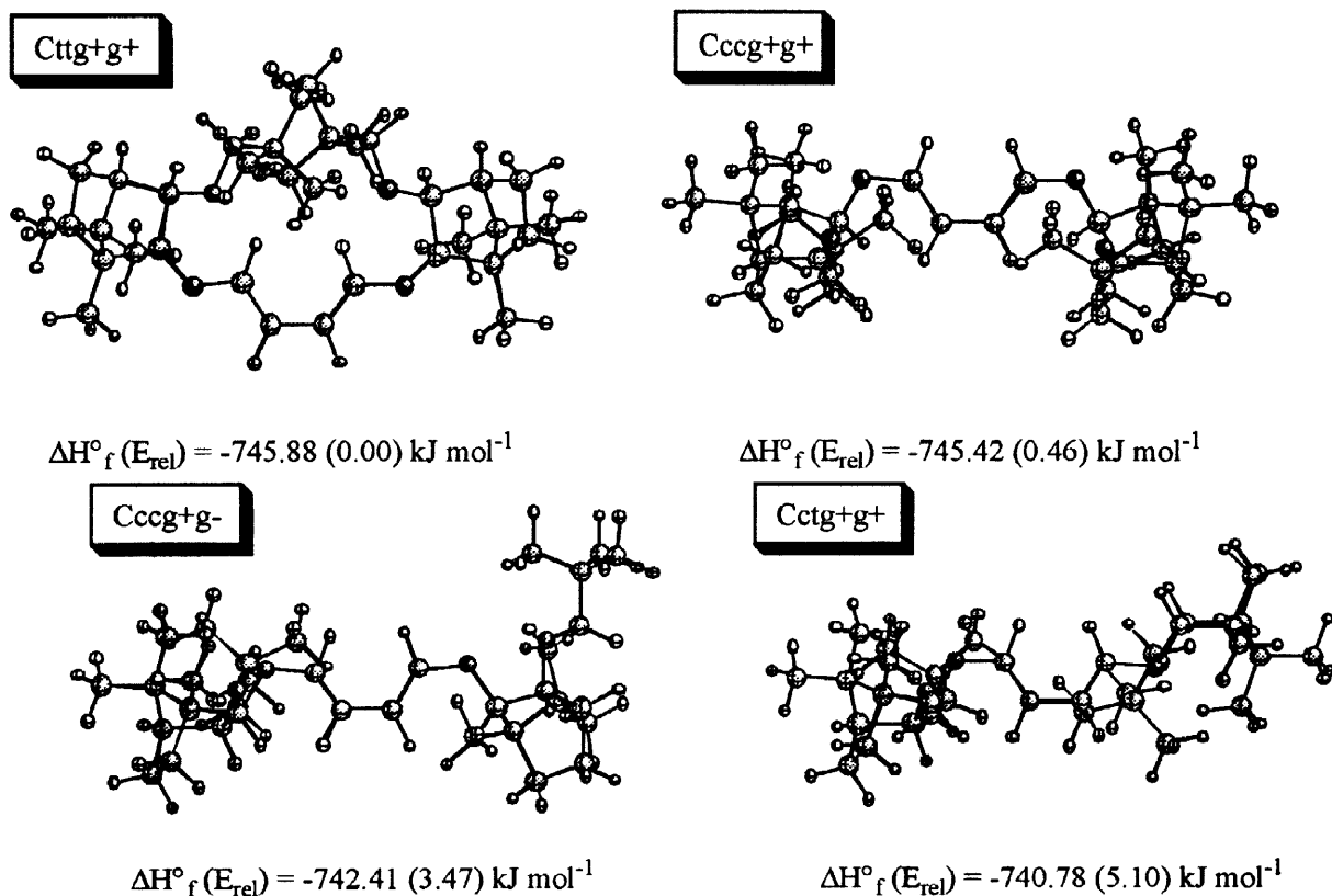
Figure 3. The four more stable cisoid conformers of ( E,E )-1,4-bis[(1 R ,2 S ,3 R ,4 S )-3-(2,2-dimethylpropoxy)-1,7,7-trimethyl bicyclo[2.2.1]heptyl-2-oxy]-1,3-butadiene ( 1d )
