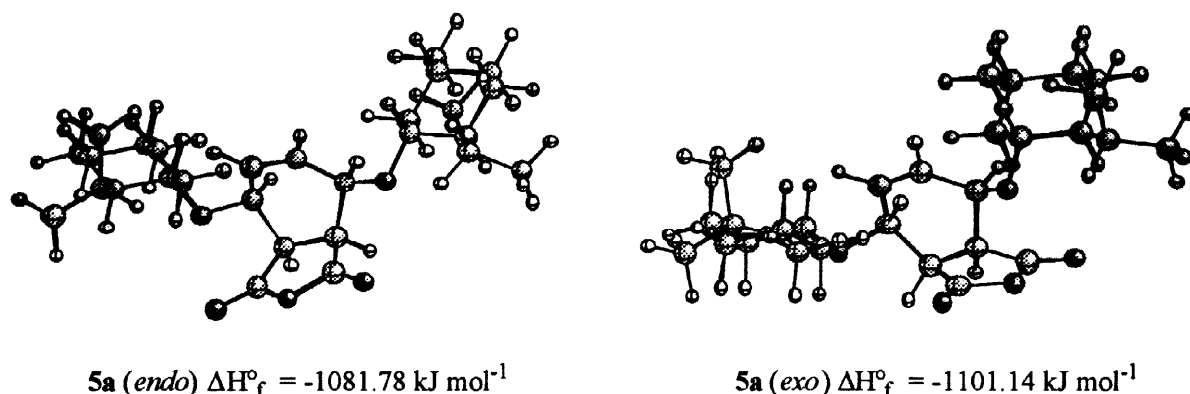
Figure 4. Lowest energy conformers (AM1) of the endo and exo stereoisomers of adduct 5a .
