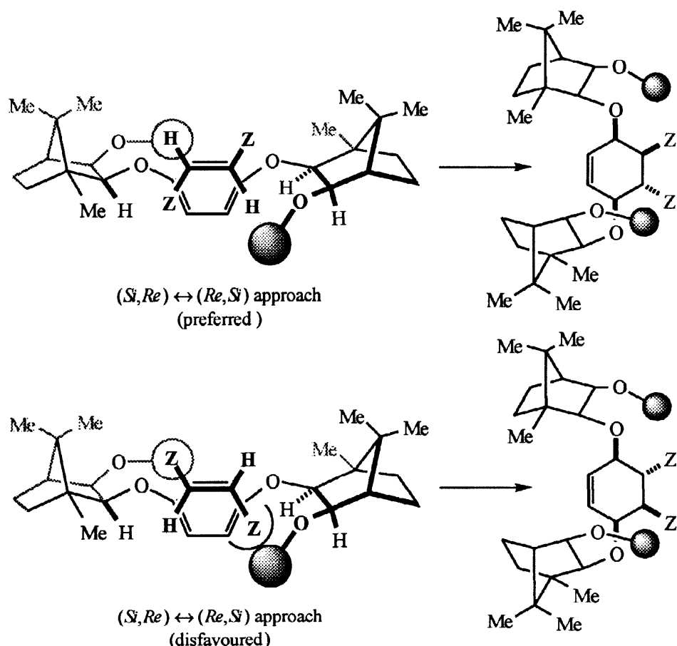
Figure 6. Predicted facial selectivity in the cycloaddition of ( E,E )-1,4-dialkoxy-1,3-diene 1d with fumaronitrile ( Z = \text{CN} ) and with diethyl fumarate ( Z = \text{CO}_2\text{Et} )
