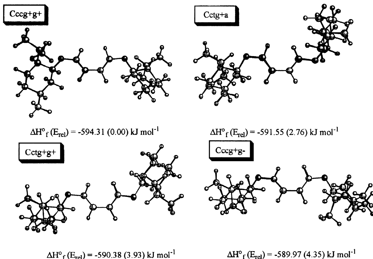
Figure 2. The four more stable cisoid conformers of ( E,E )-1,4-bis( l -menthyloxy)-1,3-butadiene ( 1a )
