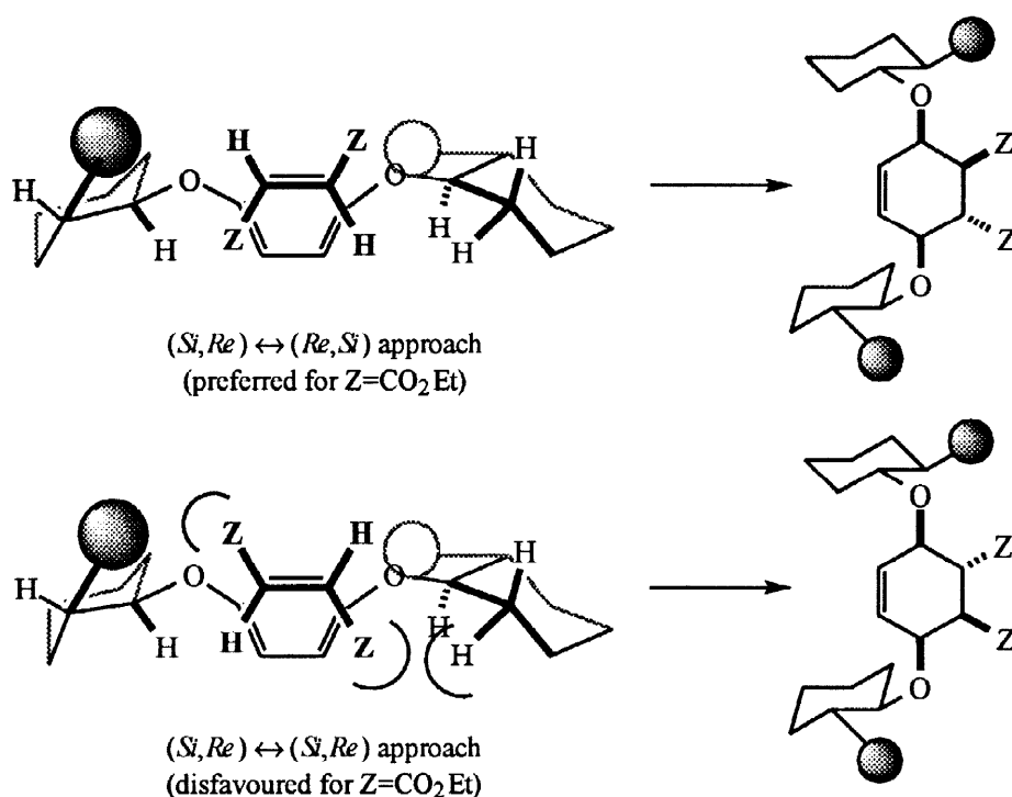
Figure 5. Predicted facial selectivity in the cycloadditions of ( E,E )-1,4-dialkoxy-1,3-dienes 1a-c with fumaronitrile ( Z = \text{CN} ) and with diethyl fumarate ( Z = \text{CO}_2\text{Et} ).
